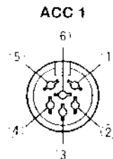
Vista del Panel Posterior TS-450S/690S/850S/950SDX
